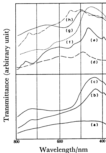
Fig. 1. Electronic absorption spectra of aromatics– \text{ZnCl}_2 complexes.
